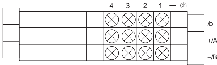
DX106 Screw-On Terminals
