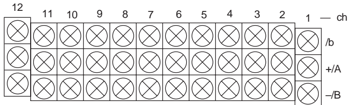
DX112 Screw-On Terminals
