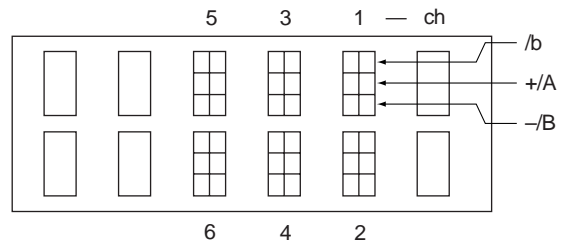
DX102, DX104, DX106 Clamped Terminals (/H2)
